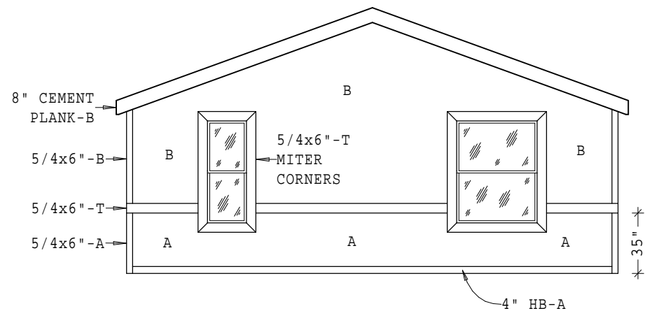
REAR ELEVATION
